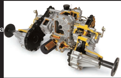
Kubota Original Transmission
